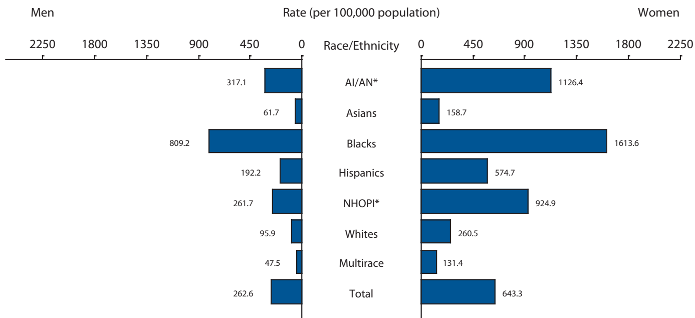
Figure L. Chlamydia — Rates by Race/Ethnicity and Sex, 2012
