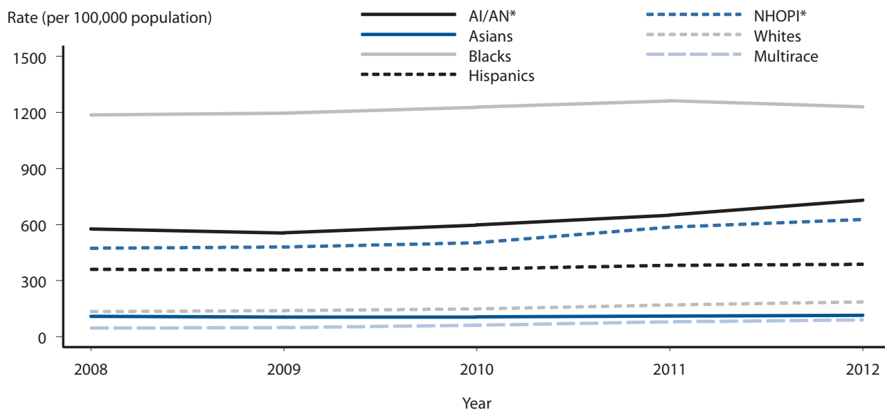
Figure 6. Chlamydia — Rates by Race/Ethnicity, United States 2008 – 2012
