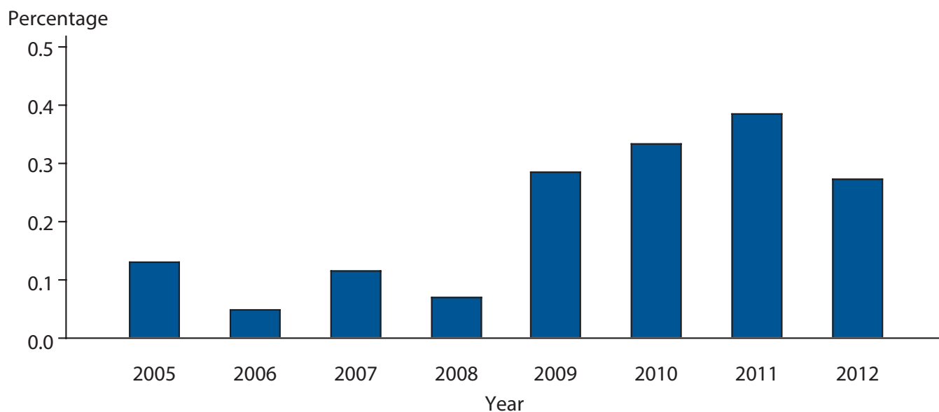
Figure 24. Percentage of Neisseria gonorrhoeae Isolates with Elevated Ceftriaxone Minimum Inhibitory Concentrations (MICs) ( \geq 0.125 \mu\text{g/ml} ), Gonococcal Isolate Surveillance Project (GISP), 2005 – 2012
