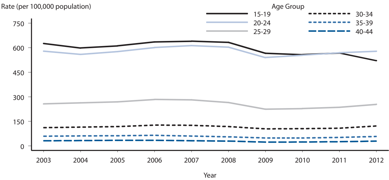
Figure 17. Gonorrhea — Rates by Age Among Women Aged 15 – 44 Years, United States, 2003 – 2012
